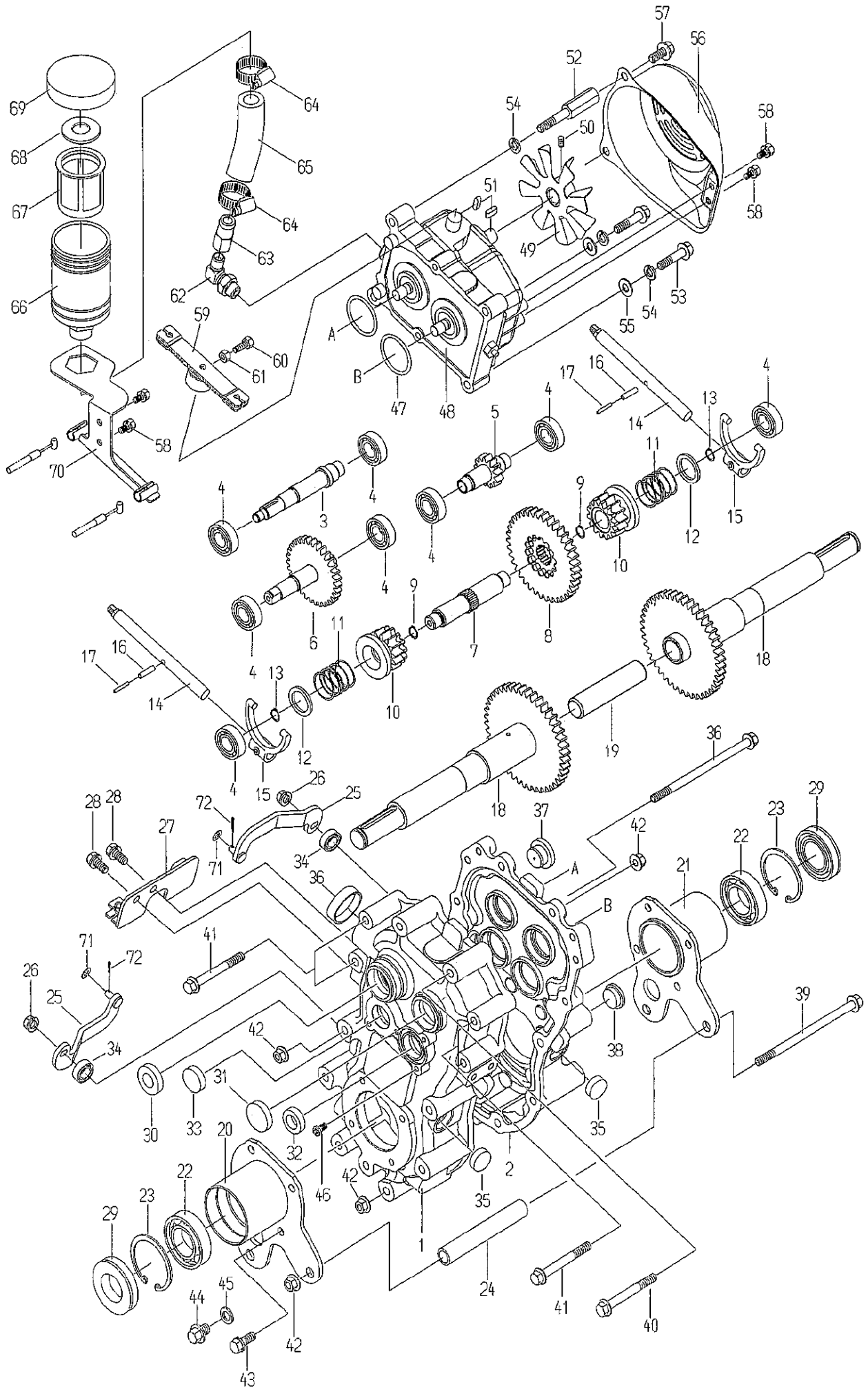
Fig. 2 TRANSMISSION
