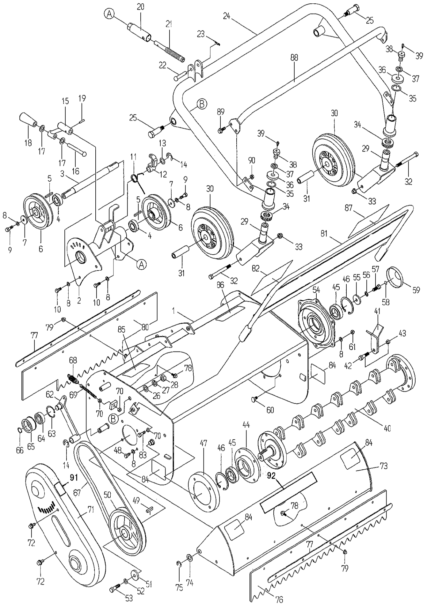
Fig. 4 ROTARY COVER
