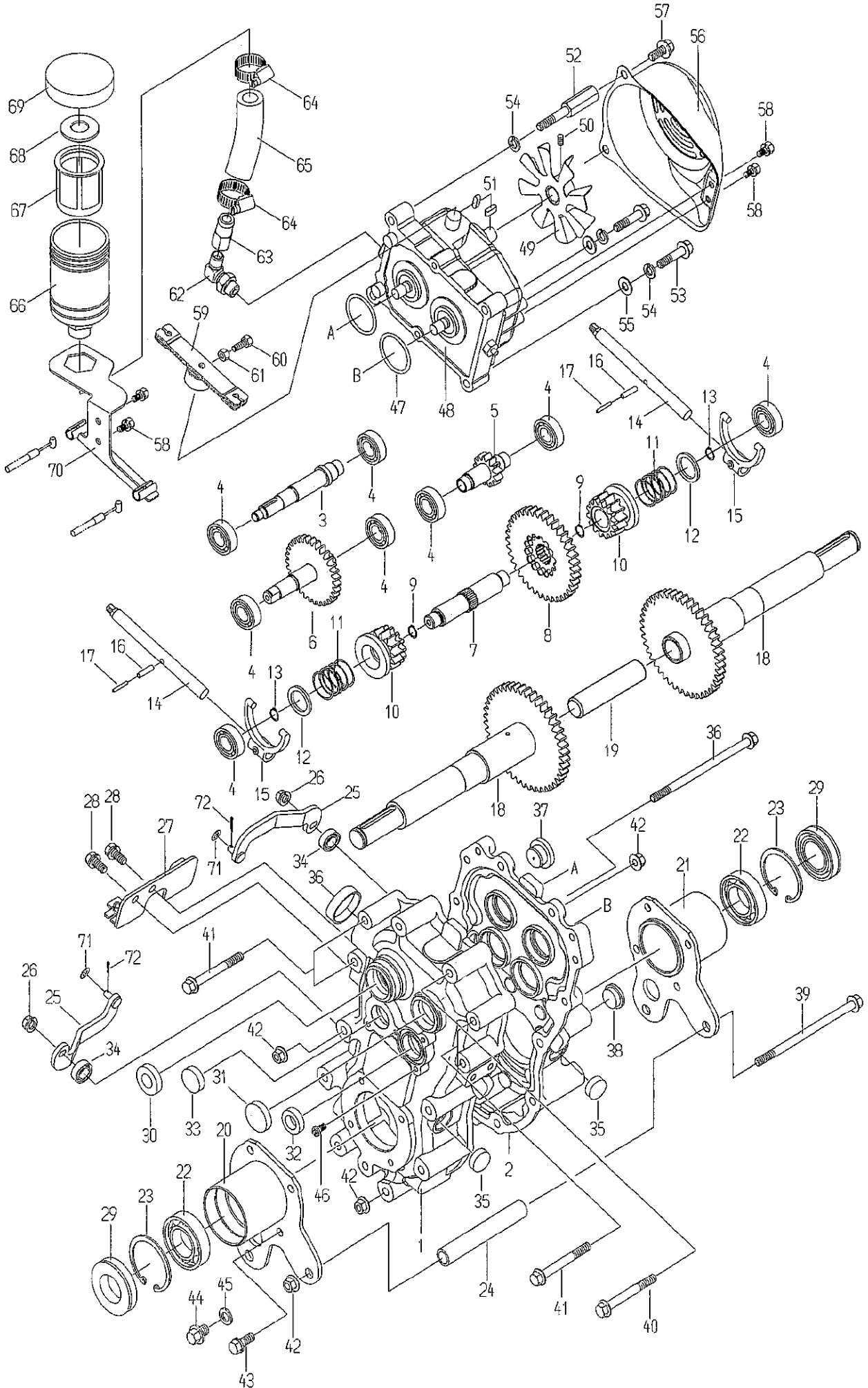
Fig. 2 TRANSMISSION
